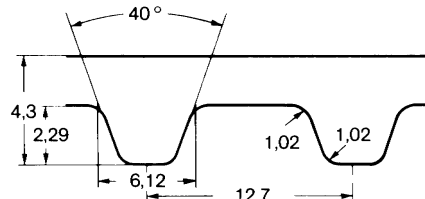
Type H (nominal dimensions – mm)
